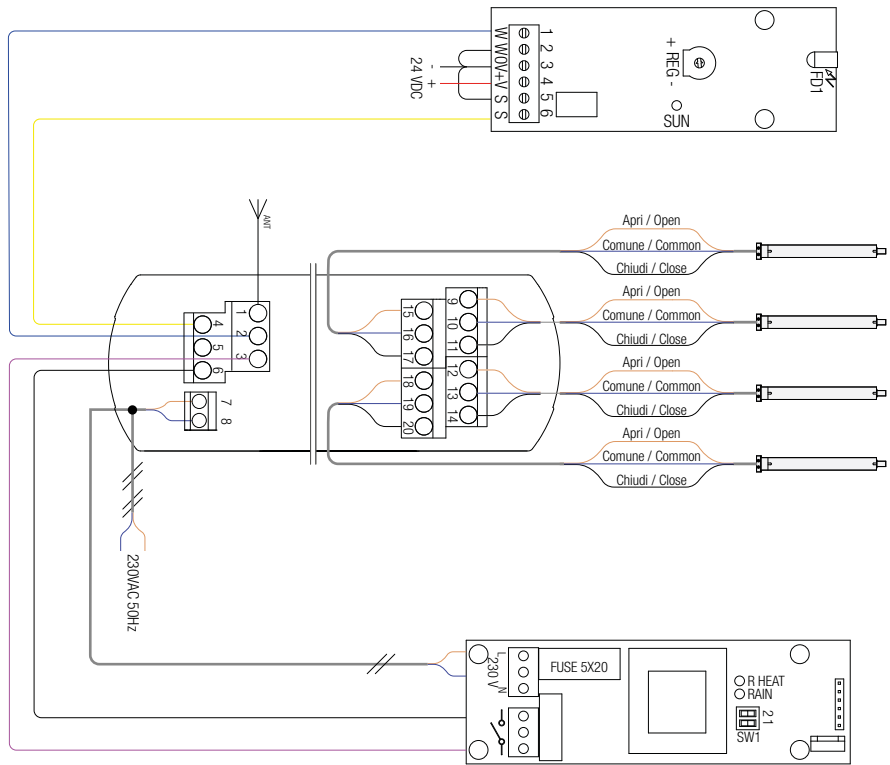
Blinds Management Scheme with an AF-850 Module
