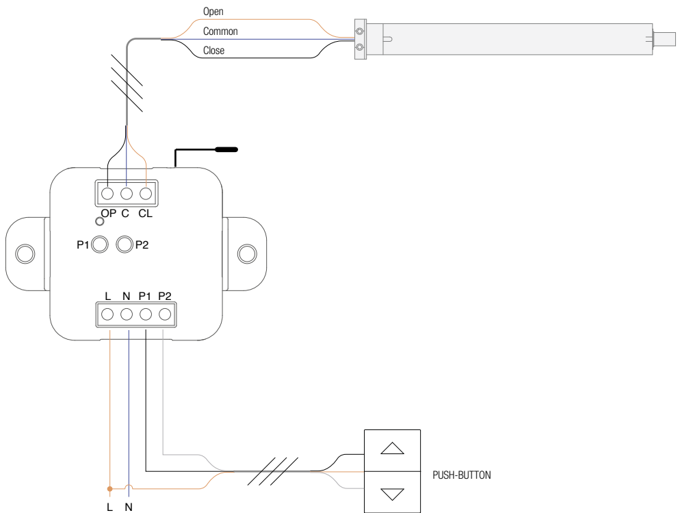
Blinds Management Scheme with an AF-820 Module
