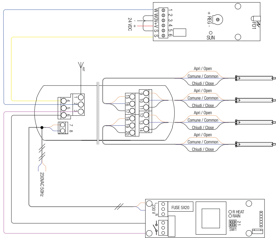
Blinds Management Scheme with an AF-840 Module
