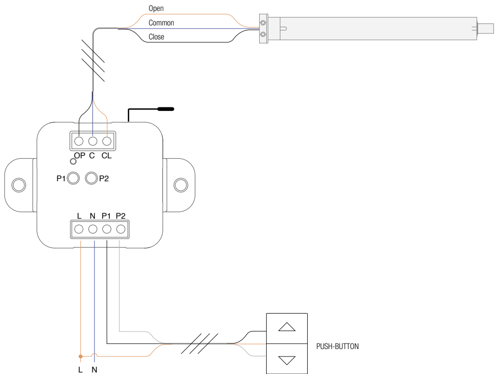
Blinds Management Scheme with an AF-800 Module
